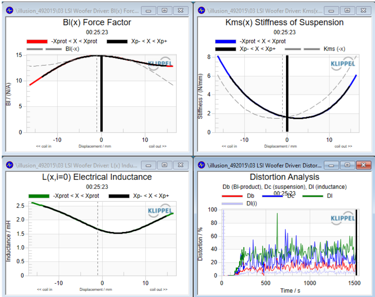
Illusion Audio C12 XL Klippel
