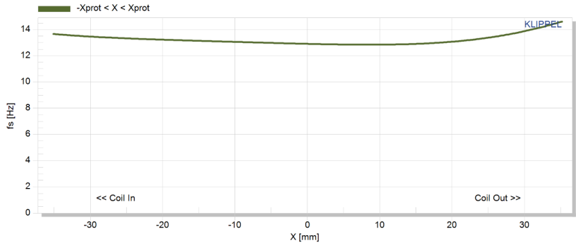
Q-factor Q_{ts}(X)
